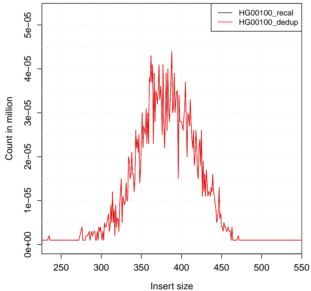
Insert size distribution
