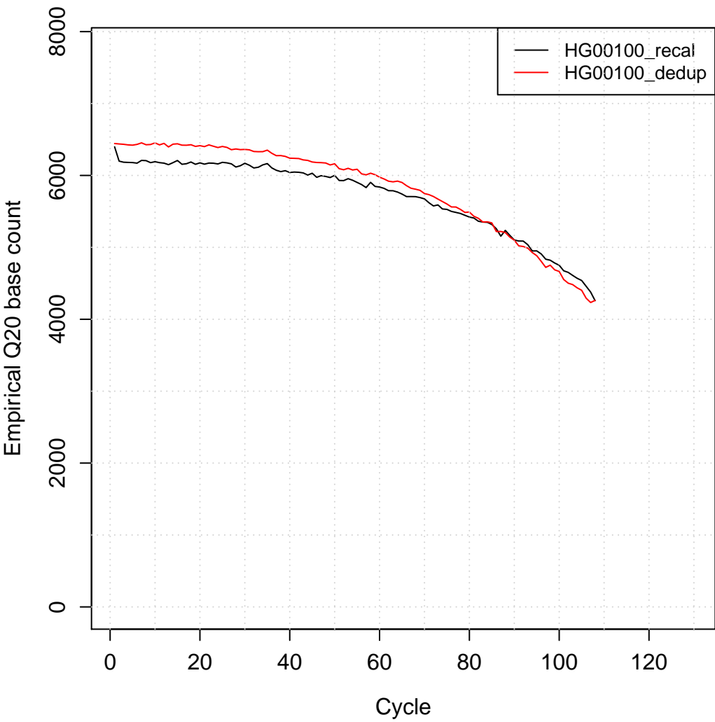
Empirical Q20 base count by cycle
