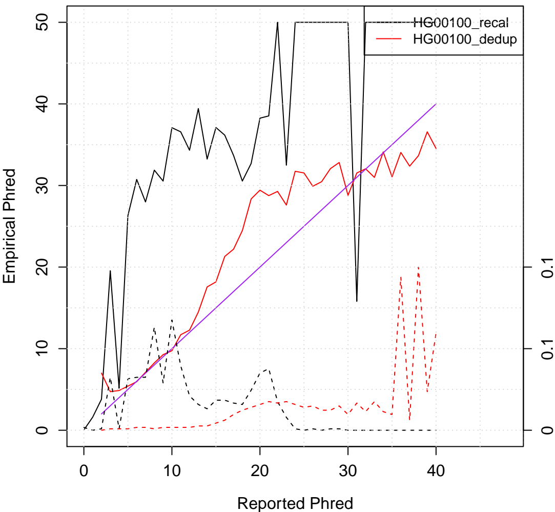
Empirical vs reported Phred score
