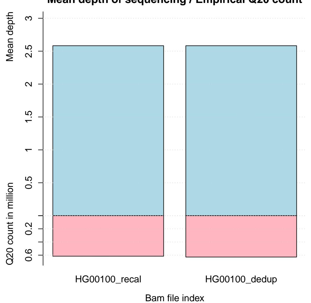
Mean depth of sequencing / Empirical Q20 count
