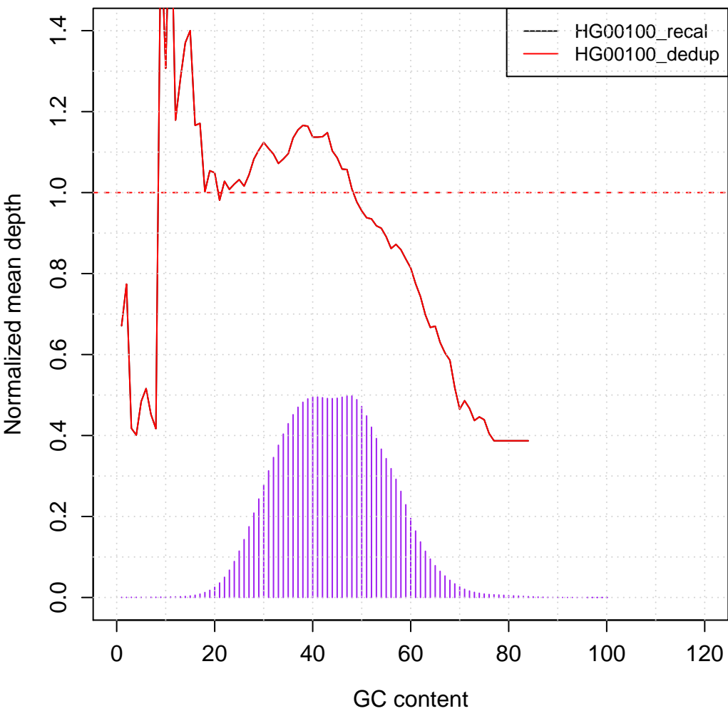
Mean depth vs. GC
