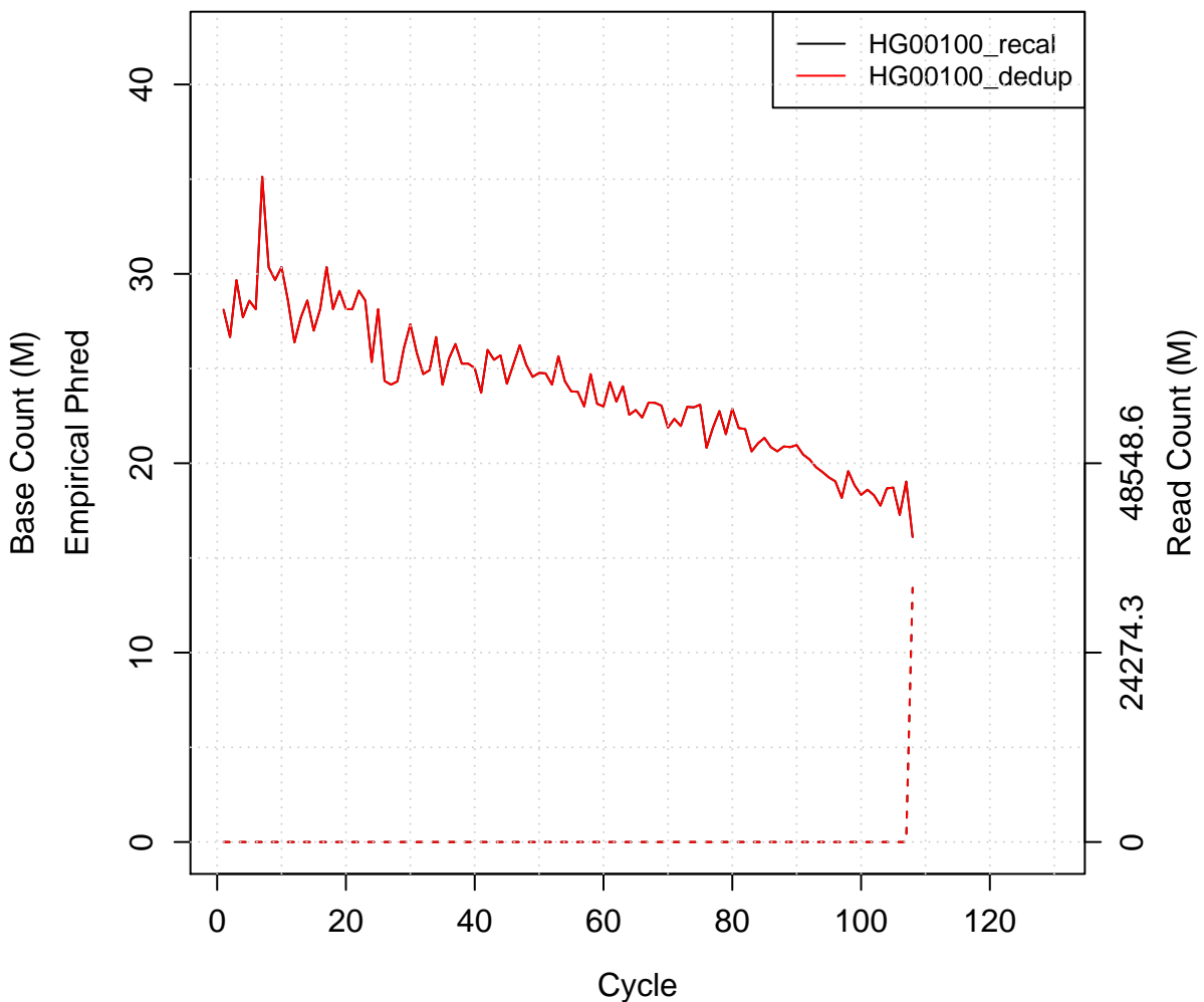
Empirical Phred score by cycle
