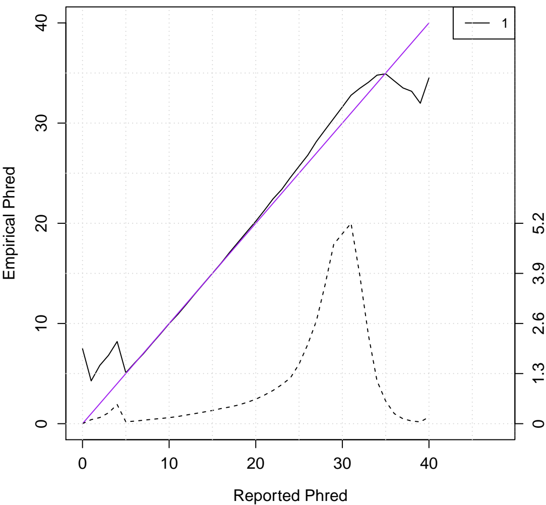
chr20:9M-10M Empirical vs reported Phred score
