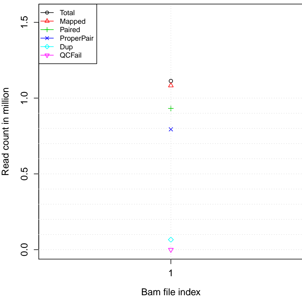
chr20:9M-10M Flag stats
