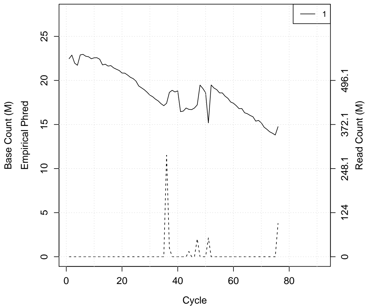
chr20:9M-10M Empirical Phred score by cycle
