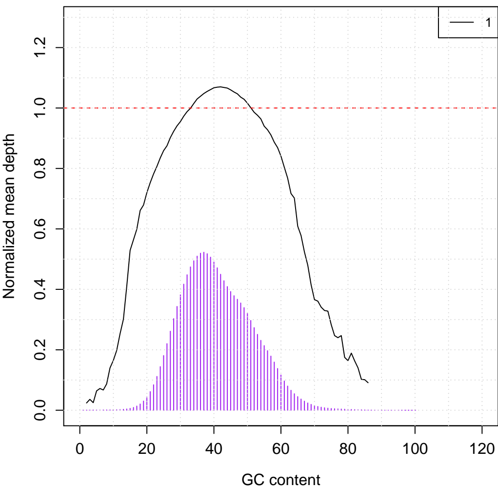
chr20:9M-10M Mean depth vs. GC
